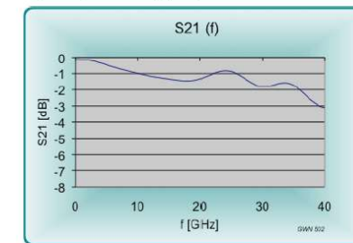
Figure 14 Insertion loss in dB
