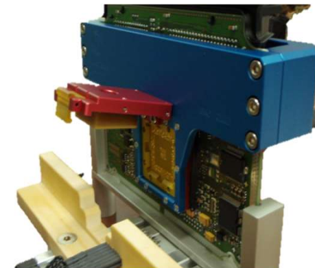
ECU test JIG
